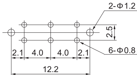
PCB DIMENSION
