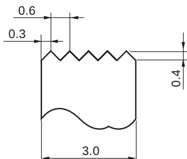
KNOB DETAIL
