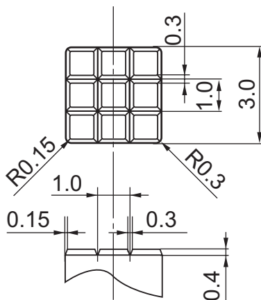
KNOB FORM
