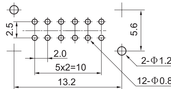
PCB DIMENSION (BOTTOM VIEW)
