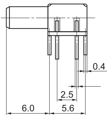
KNOB FORM
